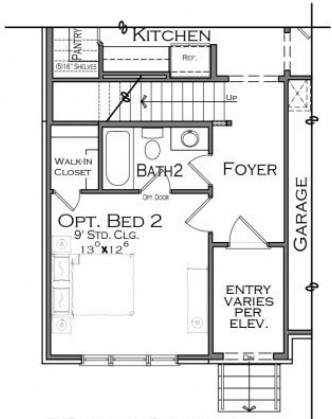
MAIN LEVEL OPTIONAL BED 2 WITH BATH & WALK-IN CLOSET OPTIONAL DOOR
