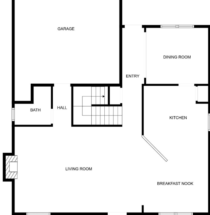
FLOOR 1
