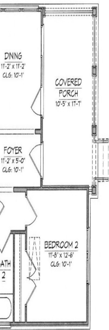
LEVEL FLOOR PLAN
