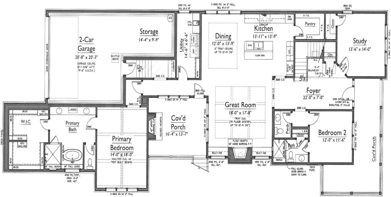
1 LOWER LEVEL FLOOR PLAN 1/8" = 1'-0"
